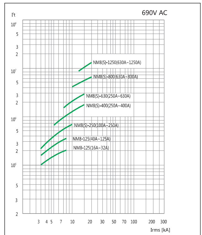
A^2s curve
