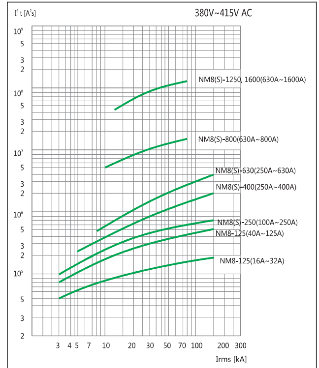
A^2s curve
